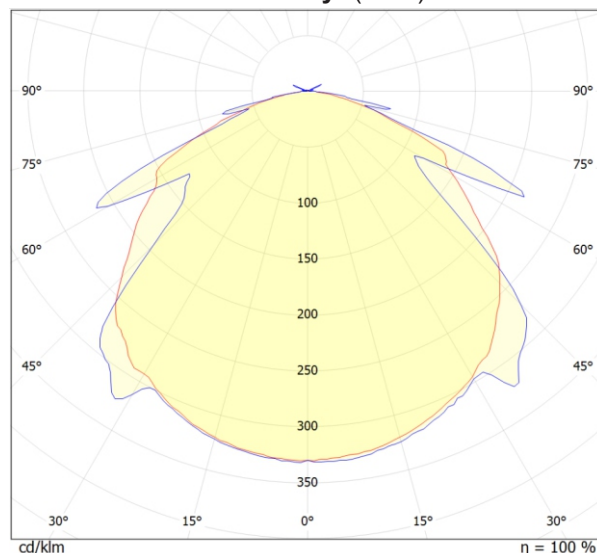
Photometry: (120°)
